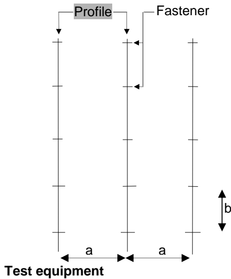
Fig. 10: Dimension of specimen
