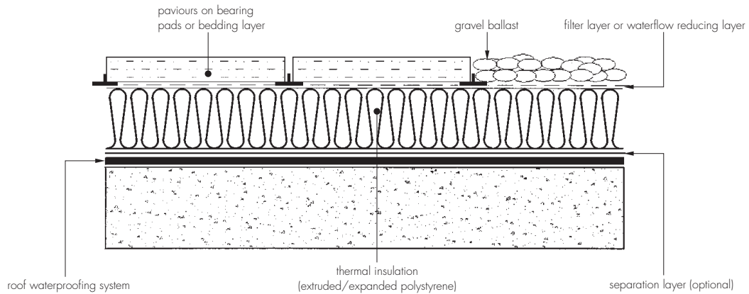
Figure 1 Schematic build-up of an inverted roof system
