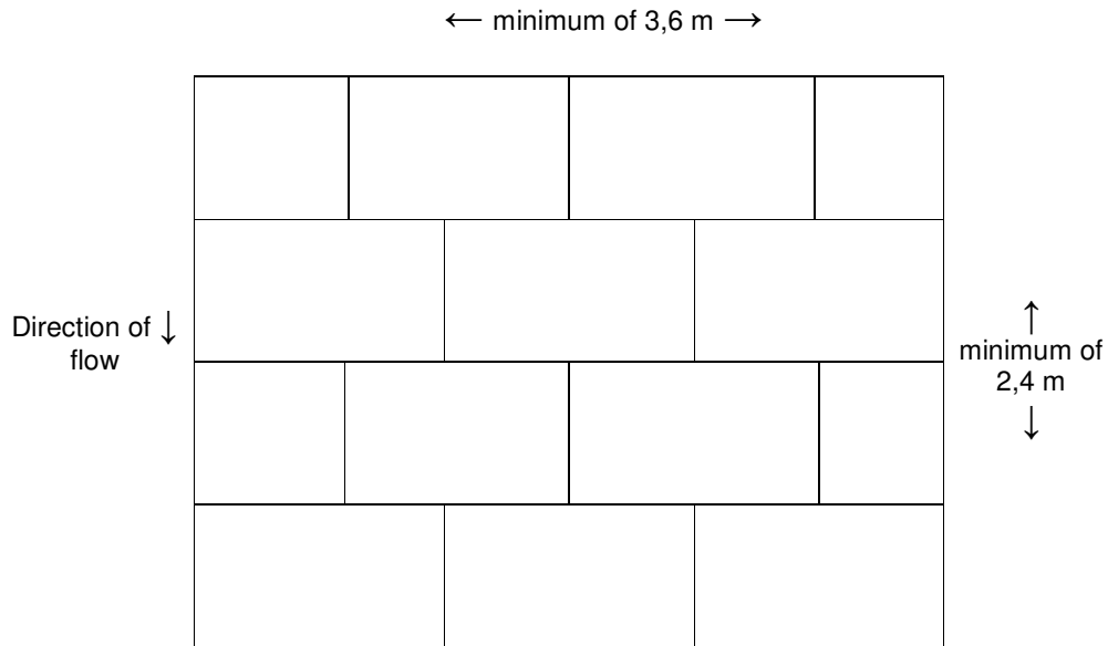
Example of board layout
