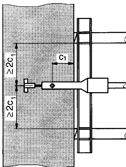
Figure A.3.1.5.2 Example of a shear test rig
