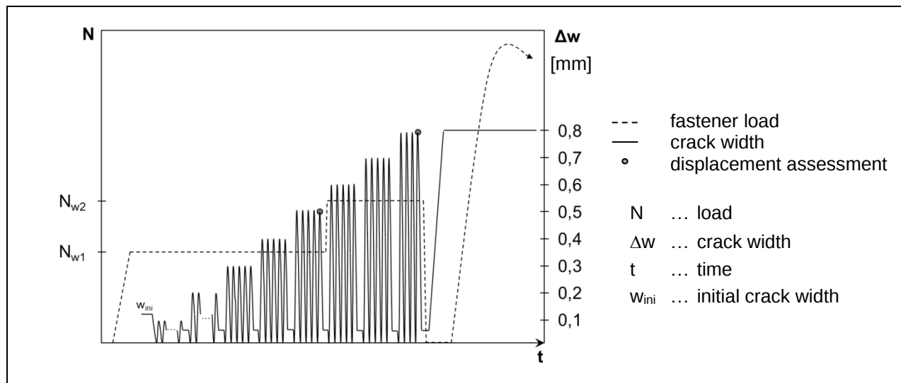
Figure 2.2.14.3.1 Schematic test procedure C2.5
