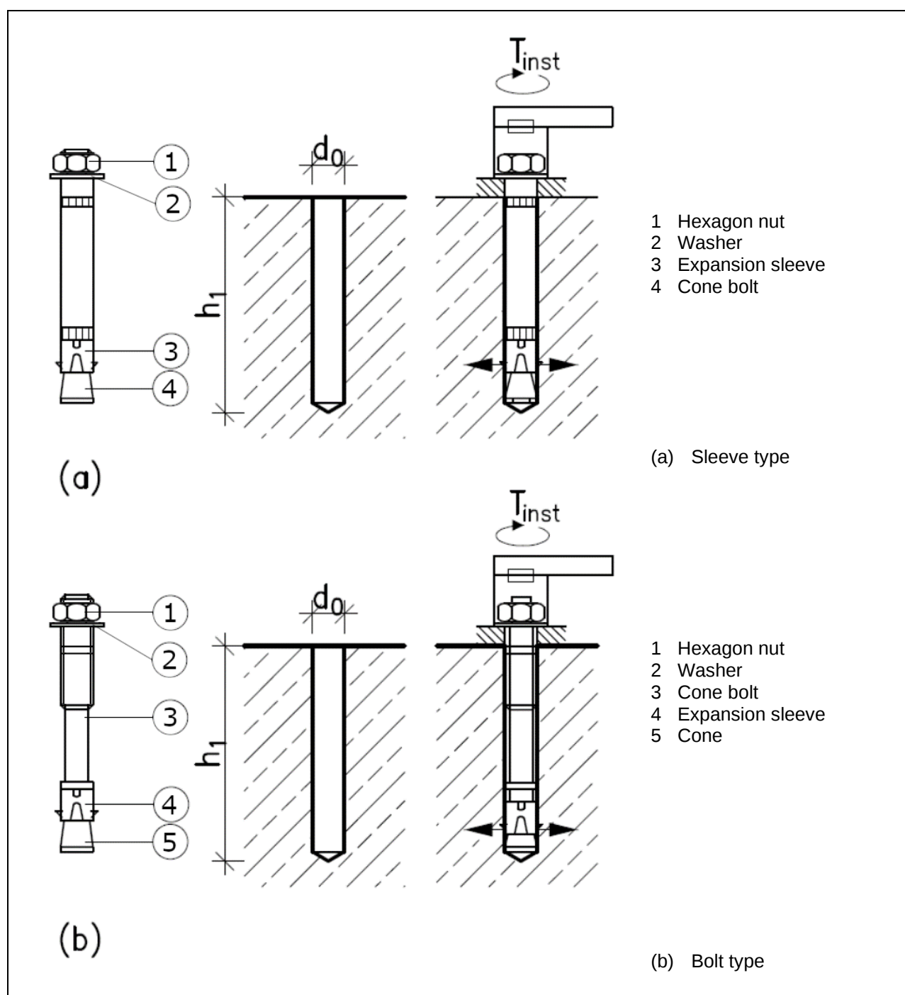
Figure 1.1.1 Example of torque-controlled expansion fasteners
