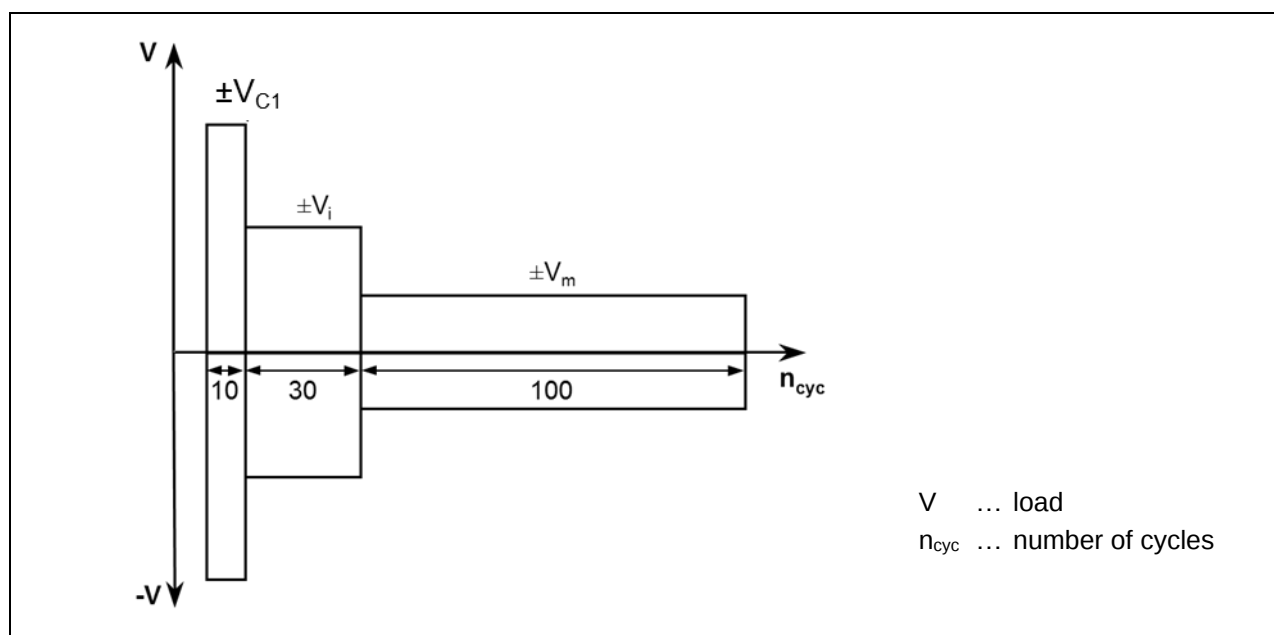
Figure 2.2.13.1 Required load history for test series C1.2
