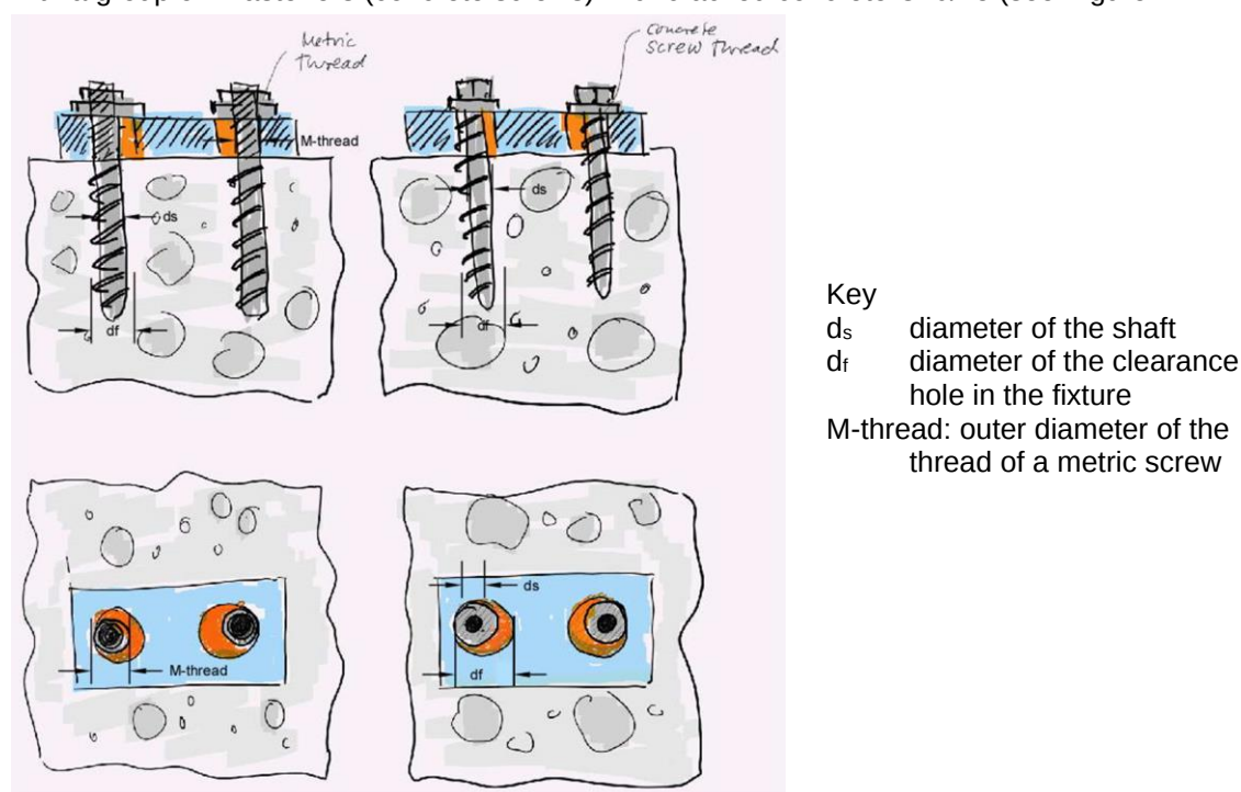
Figure 2.2.7.2.2 Most unfavourable condition - largest annular gap for direction of loading force as given in Figure 2.2.7.2.4
