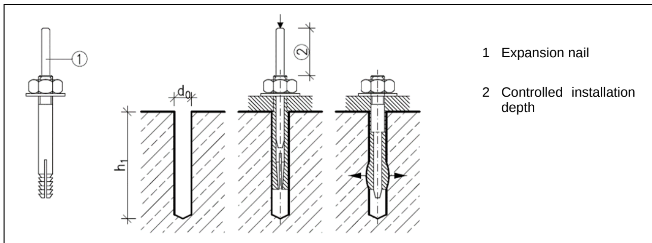
Figure 1.1.3 Shank-down type fastener (stud fastener)
