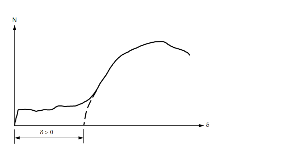
Figure A.2.5.3 Load/displacement behaviour with uncontrolled slip
