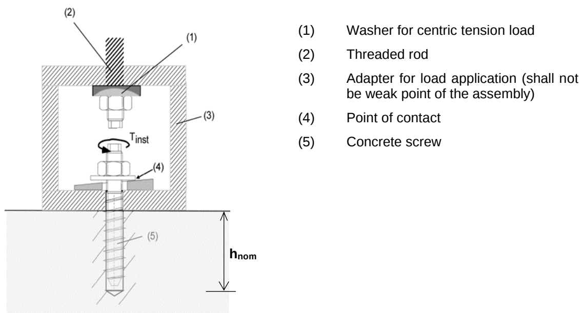
Figure A.3.3.2.2 Example of load application to concrete screws via adapter in tests F4 with repeated loads
