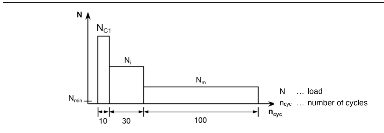
Figure 2.2.12.1 Required loading history for test series C1.1
