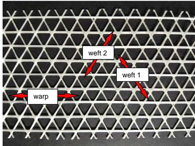
Figure A.2 Scheme of measurement of mesh size on triaxial mesh
