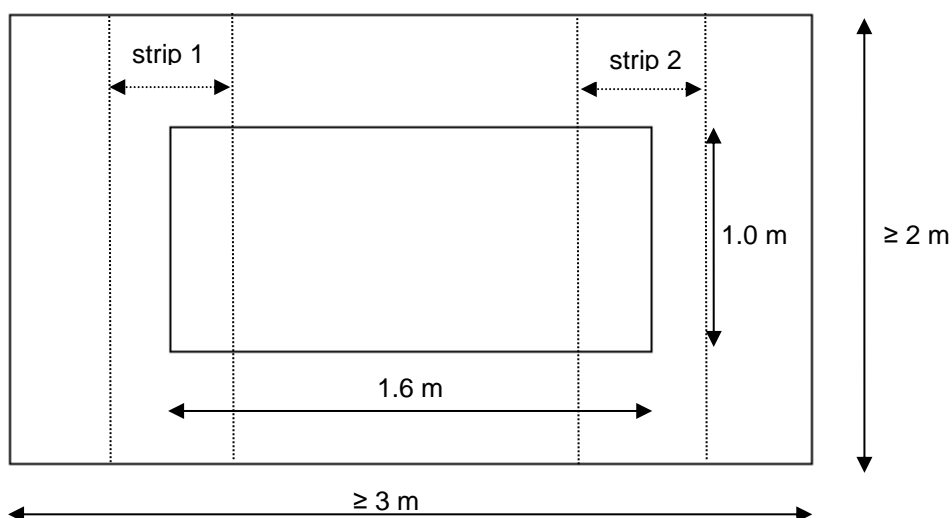
Figure C.1 - Test wall – dimensions
