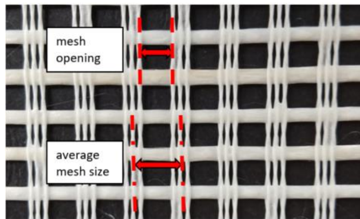
Figure 1 Relation between mesh size and mesh opening in specific case of threads consisting of more yarns
