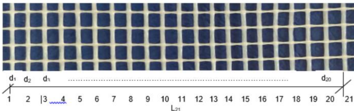
Fig. A.1 Scheme of measurement of mesh size on rectangular mesh
