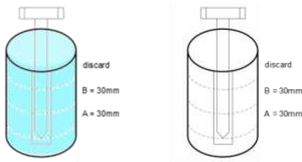
Figure 2.2.2.13.1 Example for cutting fastener samples into slices of 30 mm.
