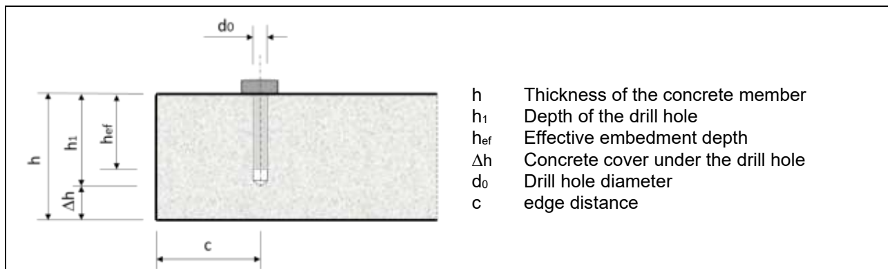
Figure 1.2.1.1 Definitions of dimensions for installation
