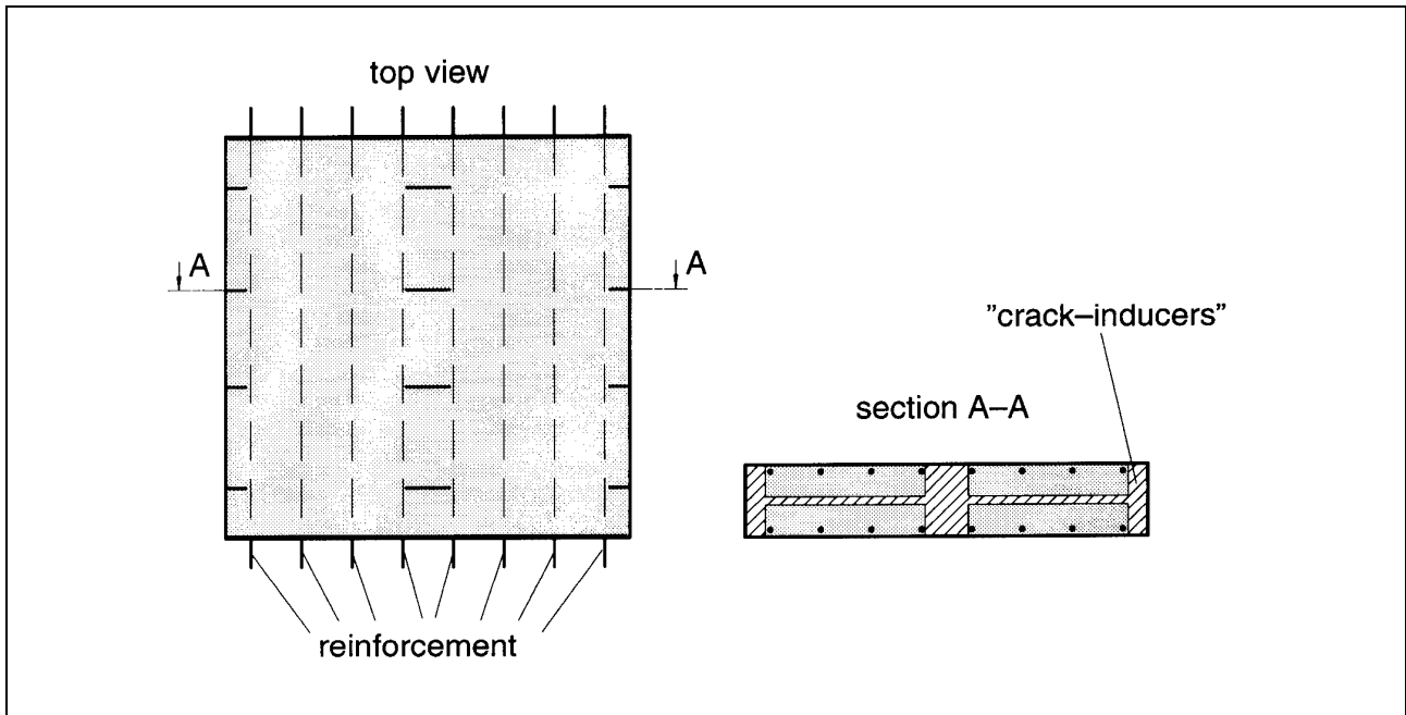
Figure 2.2: Example of a test member for plastic anchors tested in cracked concrete
