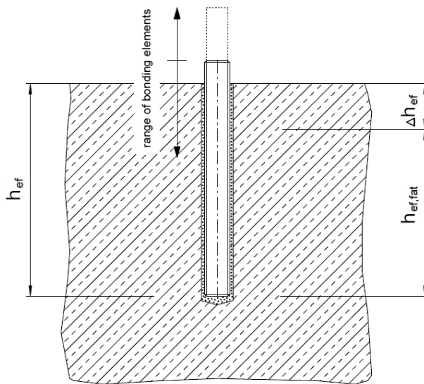
Figure 2.1 Effective embedment depth h_{ef,fat} of bonded fasteners
