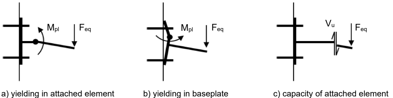
Figure 6.1: Seismic design by protection of the fastening
